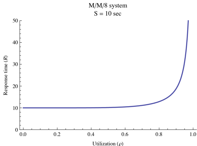
Exhibit 8. This curve relates response time as a function of utilization for an M/M/8 system.
